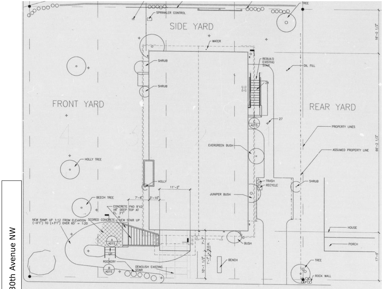
Figure 35: Site plan from 1999 renovation project, R.G. Satterwhite, Triangle Works. Sunset Hill Community Hall archives.
