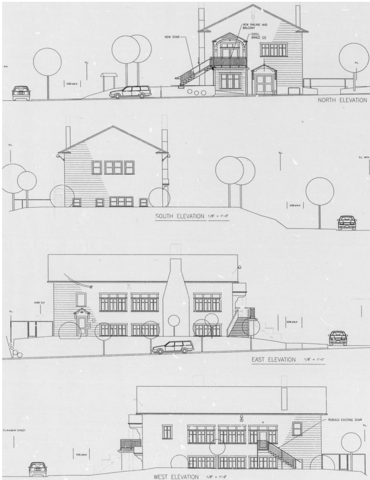
Figure 36: Elevation drawings, 1999 renovation project, R.G. Satterwhite, Triangle Works. Sunset Hill Community Hall archives.
