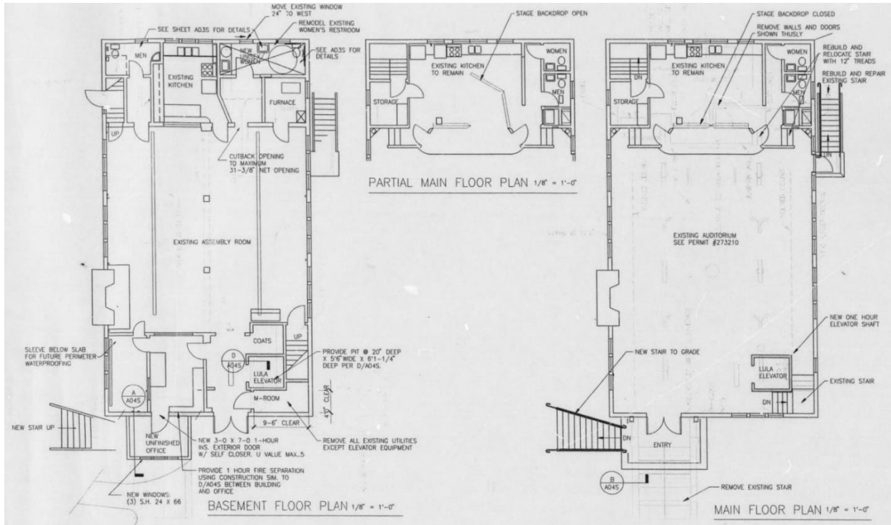
Figure 37: Floor plans, 1999 renovation project, R.G. Satterwhite, Triangle Works. Sunset Hill Community Hall archives.
